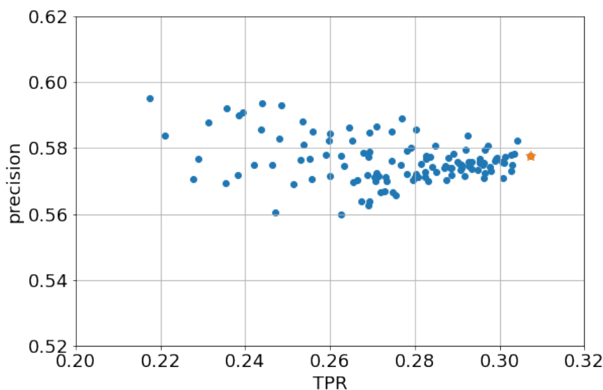
Figure 3. Precision/TPR for S_{obs} for a number of different distance thresholds. The starred point is the one we chose, corresponding to the thresholds in Eq. 3.
