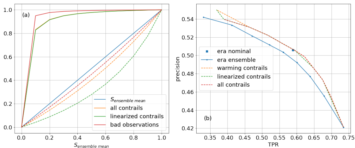
Figure 6. (a) Same as Fig. 4 but including the different choices of TPR/FPR outlined in Table 3. For each case solid lines show S_{hybrid(observed)} and dashed lines show S_{hybrid(not\ observed)} . (b) Same as Fig. 5(a), but the dashed lines show different S_{hybrid} for the different cases in Table 3.
